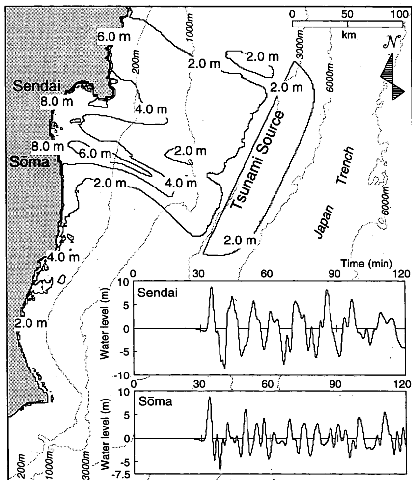
Fig. 3 Results of the numerical simulation of the Jōgan tsunami. Based on historical documents and proposed fault parameters of the Jōgan tsunami (Satō, 1989), a model of the tsunami source was established. The computational region covers the area 37°N to 39°N and 143°E to 144°30'E. An interval of 2 s and spatial grid size of 1 km were used. The simulation covers wave propagation for 5 hours. The maximum water-elevation contours and the time history of the water levels at Sendai and Sōma are shown for 2 hours. After 30 min, a tsunami with waves 8 m high struck the Sendai plain. Thin dotted lines show submarine contours in meters of depth.
