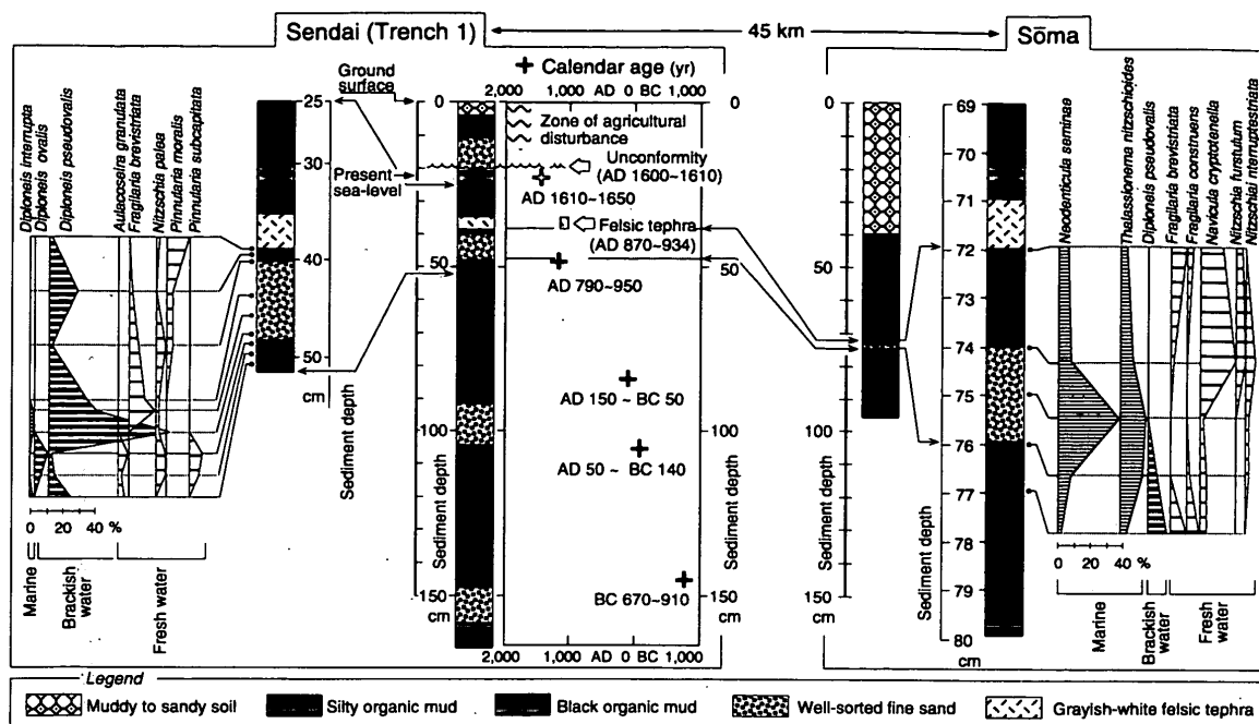
Fig. 2 Stratigraphic and paleontological correlation of the sedimentary sequences of Sendai (Trench 1) and Sōma. Fossil diatoms in the sediments indicate that sand layers of marine to brackish water origin were deposited in a back marsh environment. The thin layer of grayish-white felsic tephra at Sōma corresponds mineralogically and chemically (Fig. 1C) to that of Sendai. It follows that the sand layer just beneath the tephra is a trace of the invasion of the Jōgan tsunami. The Sendai plain was opened to agriculture about 400 years before by a feudal lord. Agricultural disturbance of the subsurface layers reaches a depth of 10 to 20 cm at Trench 1, resulting in the formation of an unconformity just below the uppermost sand layer. Some historical documents report that cultivation was interrupted by invasion of the 1611 Keichō tsunami. The calendar periods of the sand layers are estimated by the ^{14}\text{C} ages of wood fragments and indicate that the largest-scale tsunami struck the Sendai plain at intervals of about 1000 years.
